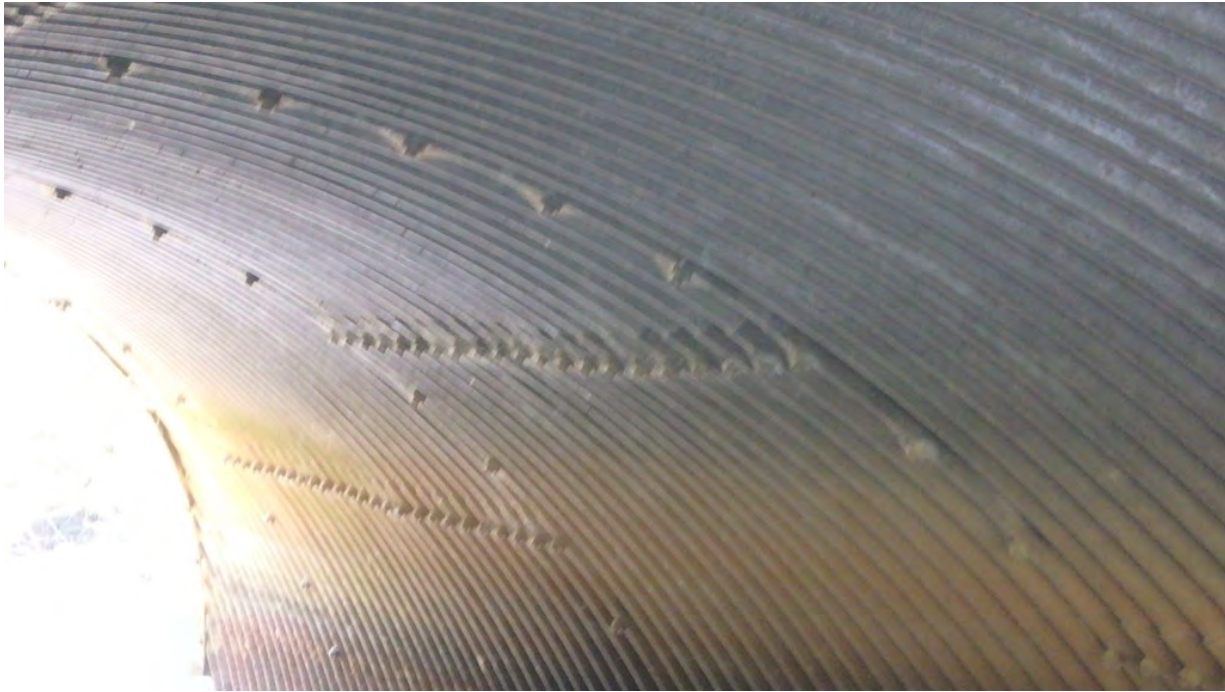
Figure 9 Deformation at Multiplate Joint
